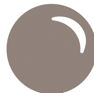
340 cappuccino
